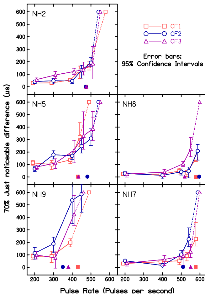
Figure 2: ITD-JNDs as a function of pulse rate in separate panels for each subject. The parameter is the CF. Non-determinable JNDs are arbitrarily plotted at 600 \mu s. Error bars represent bootstrapping 95% confidence intervals. The filled symbols at the bottom denote the inflection points of the functions JND vs. rate (see text).
