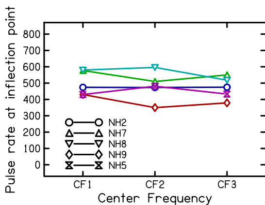
Figure 3: For each subject the pulse rate at the inflection point is shown as a function of the CF.
