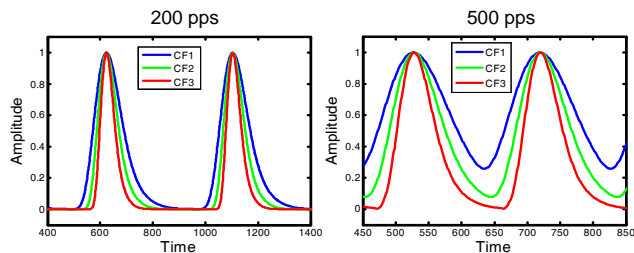
Figure 1: Envelopes of the pulse trains after passing auditory filters at the three CFs at 200 pps (left panel) and 500 pps (right panel). With increasing CF, the amount of modulation increases, in particular at the higher pulse rate.
