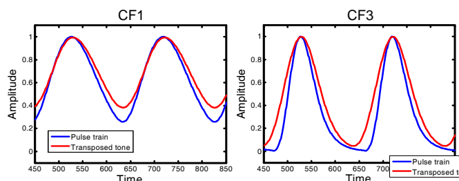
Figure 4: Envelopes of pulse trains (present study) and transposed tones [3] after passing auditory filters at CF1 (left panel) and CF3 (right panel). The pulse rate is 500 pps.
